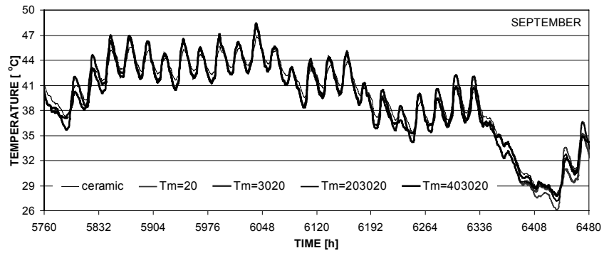
Figure 19. Internal surface temperature – September
