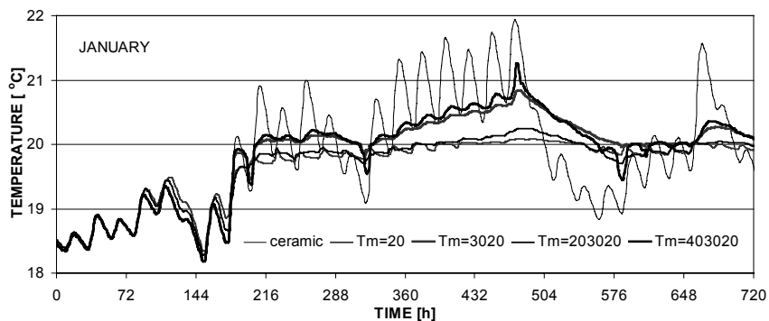
Figure 11. Internal surface temperature – January
