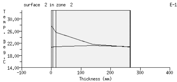
Figure 4. Temperature distribution through the ordinary ceramic wall
