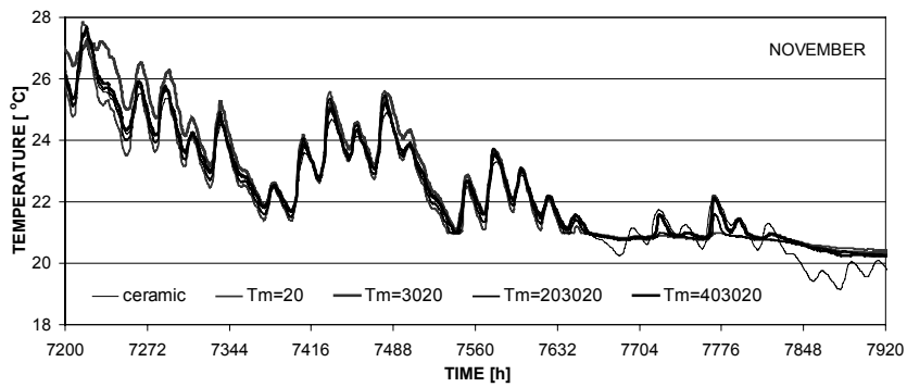
Figure 21. Internal surface temperature – November
