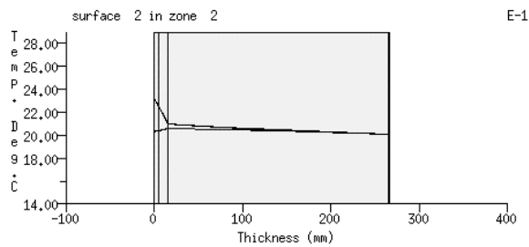
Figure 5. Temperature distribution through the PCM-composite wall
