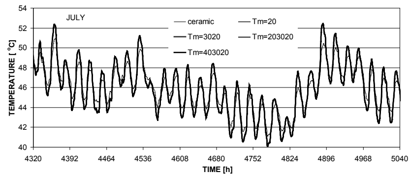
Figure 17. Internal surface temperature – July
