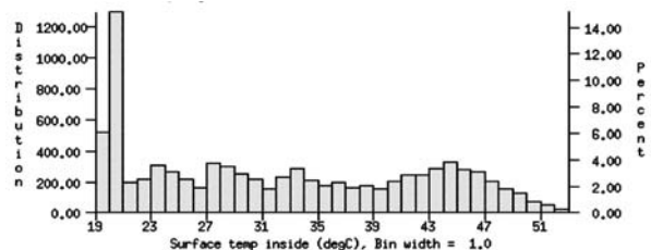
Figure 10. PCM T_m=40,30,20^\circ\text{C}
