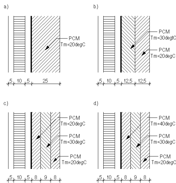
Figure 2. Configuration of multi-layered walls
