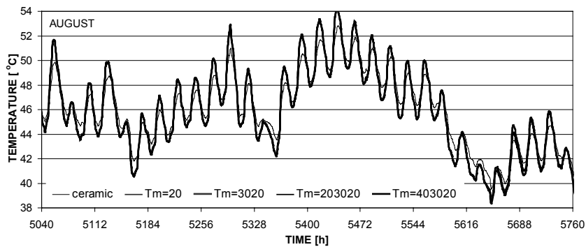
Figure 18. Internal surface temperature – August
