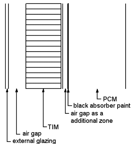
Figure 1. Cross-section through TIM-PCM wall
