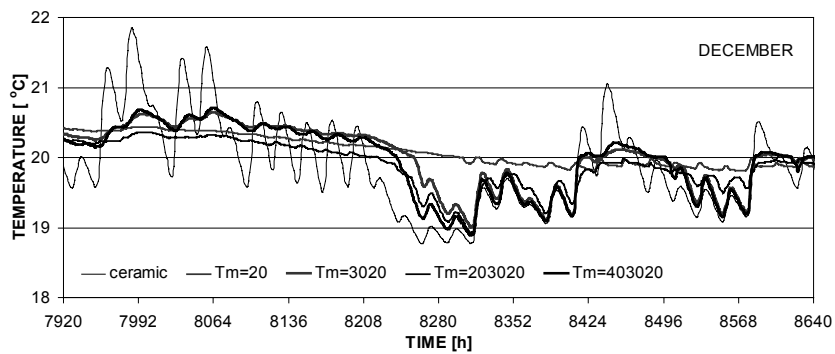
Figure 22. Internal surface temperature – December
