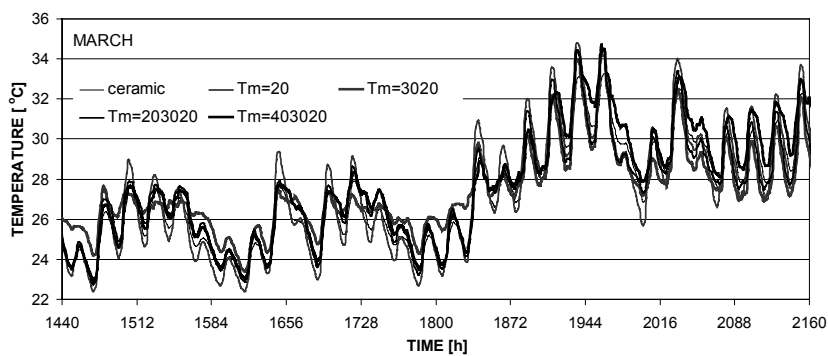
Figure 13. Internal surface temperature – March
