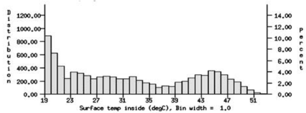
Figure 6. Ordinary ceramic
