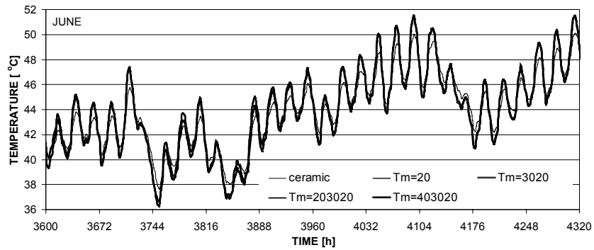
Figure 16. Internal surface temperature – June
