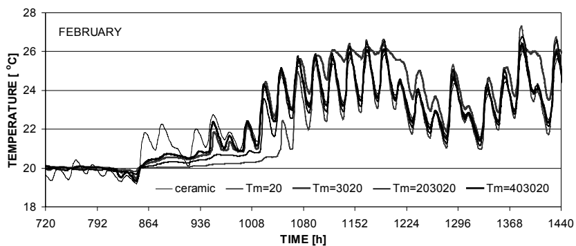
Figure 12. Internal surface temperature – February
