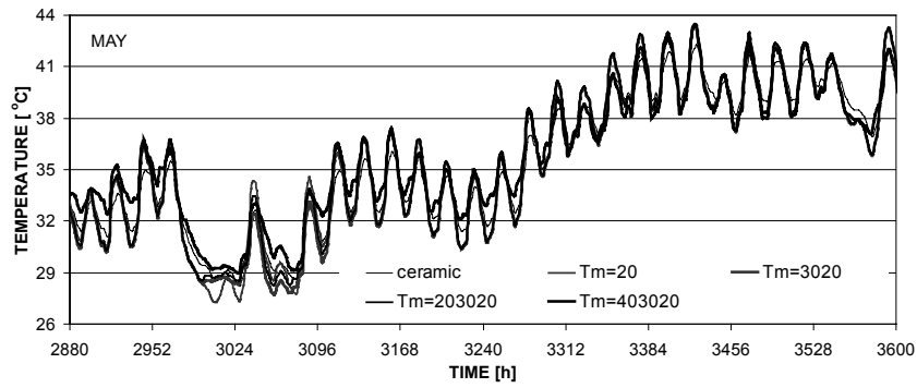
Figure 15. Internal surface temperature – May
