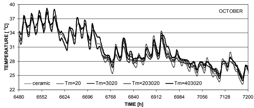
Figure 20. Internal surface temperature – October
