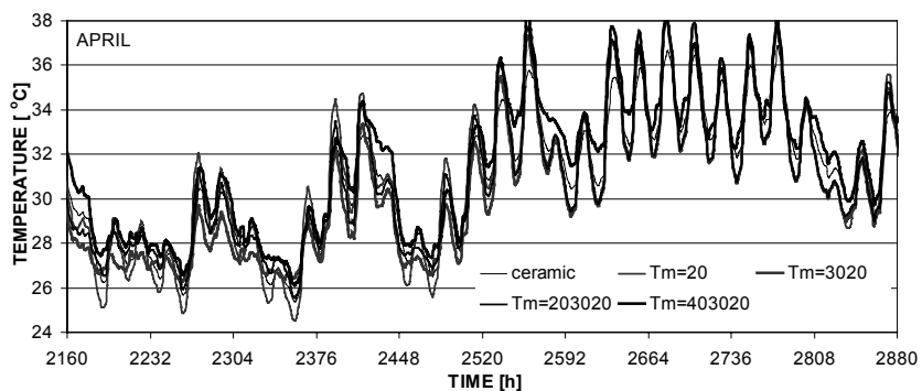
Figure 14. Internal surface temperature – April
