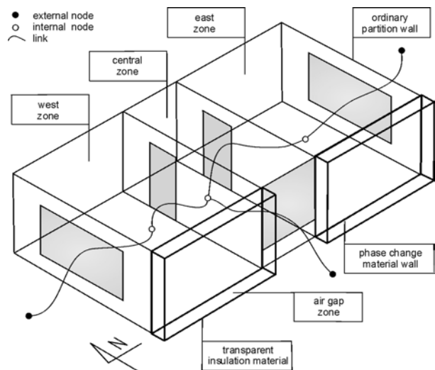
Figure 3. Schematic, prospective view of geometry and air flows in analyzed triple zone building
