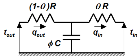
Figure 3: 2RIC wall model including two no dimensional parameters \theta and \phi .
