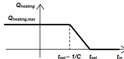
Figure 13: Feedback proportional control law
