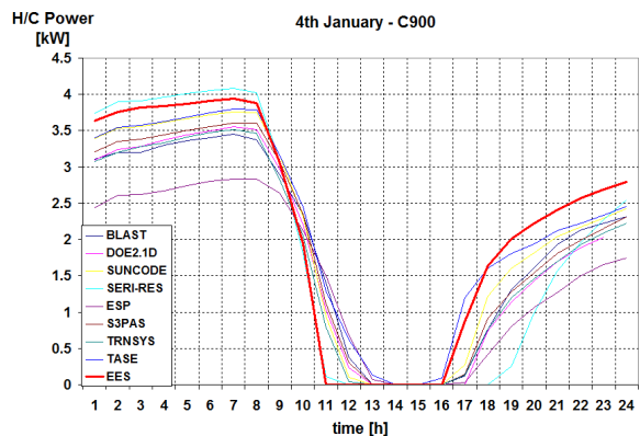
Figure 10 : C900 – 4 th January, H/C powers
