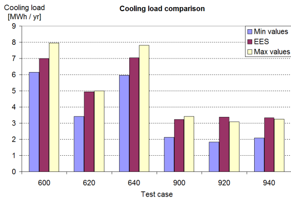
Figure 8 : C600 to C940 – Annual Cooling Demands
