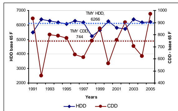
Figure 4: HDD and CDD for Hartford from 1991-2005
