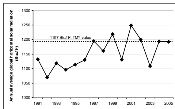
Figure 5: AvgGlo data for Hartford from 1991-2005
