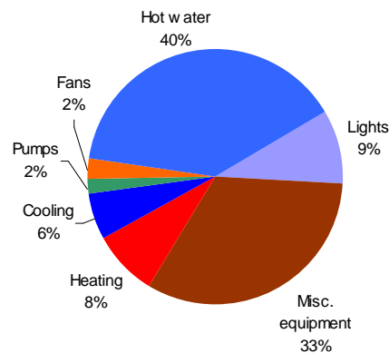
Figure 6: Annual energy consumption (all electric) breakdown by percentages
