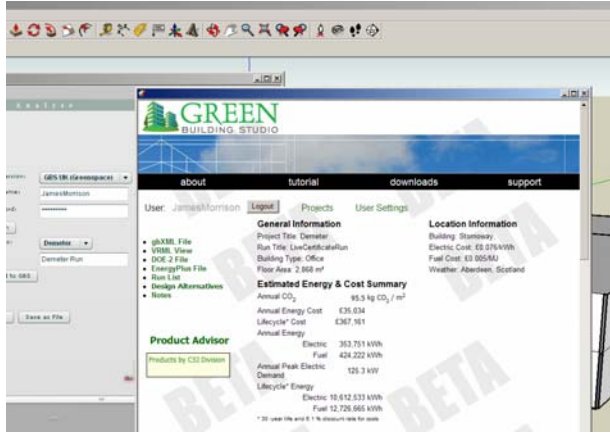
Figure 5 Demeter plugin – energy analysis report retrieved from the web service
