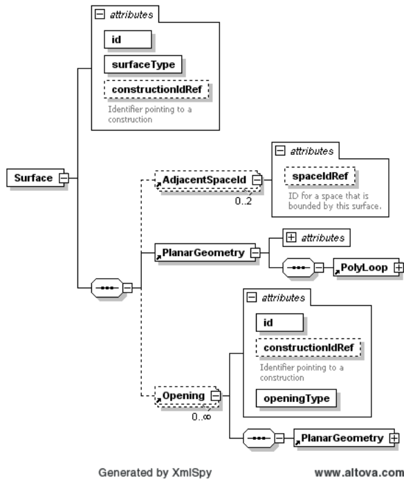
Figure 2 gbXML schema – Surface element
