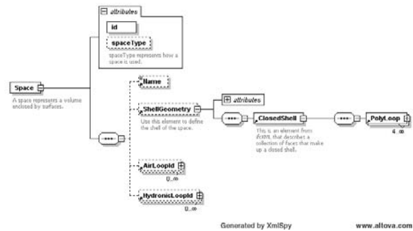
Figure 3 gbXML schema – Space element (partial representation)
