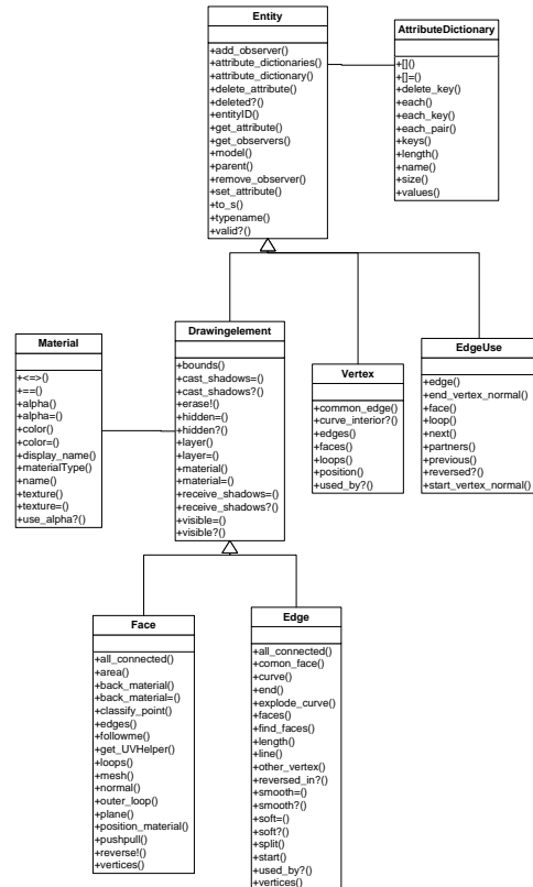
Figure 1 SketchUp application programming interface
