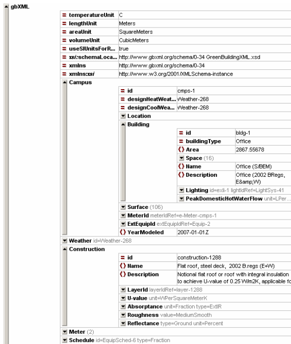
Figure 4 gbXML model
